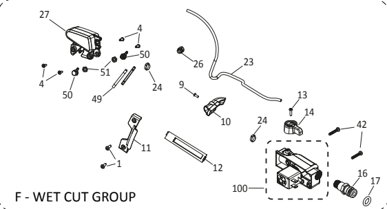
F - WET CUT GROUP
