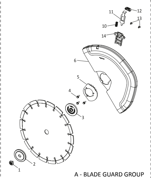
A - BLADE GUARD GROUP
