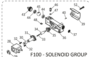
F100 - SOLENOID GROUP
