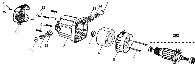
D - MOTOR GROUP
