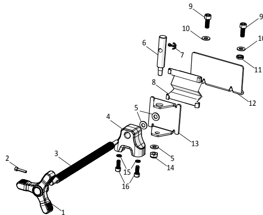
F - CLAMP GROUP
