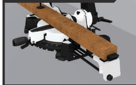
STEP 3: FOLDING END-STOP
